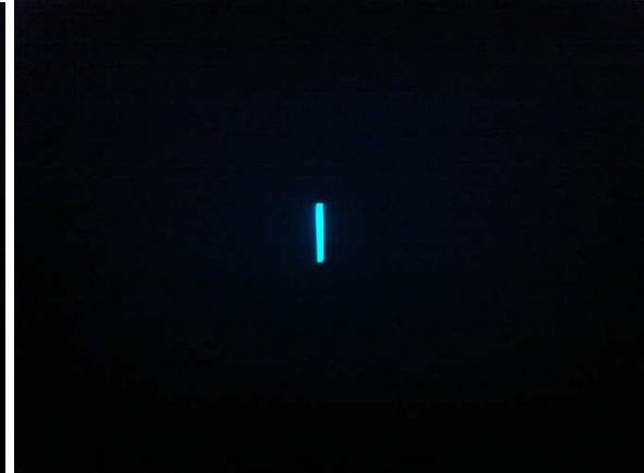
501nm ([OIII])
